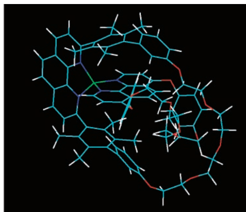
Figure 6. PM3 calculated minimum structure of [\text{Cu}(\mathbf{1})(\mathbf{3b})]^+ .
