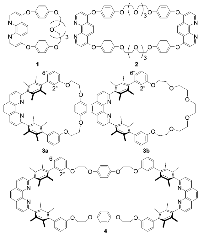
Figure 2. Macrocyclic phenanthrolines with exotopic and endo-topic coordination sites.
