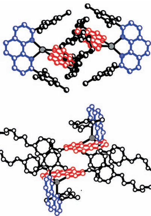
Figure 4. X-ray structure of [\text{Cu}_2(\text{2})(\text{9})_2]^{2+} (view from two sides).
