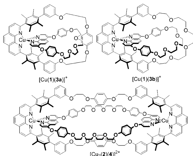
Figure 5. Ring-in-ring structures.
