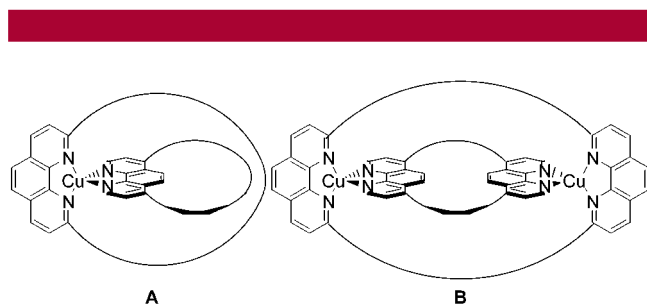
Figure 1. Pictorial representation of mononuclear and dinuclear ring-in-ring structures.
