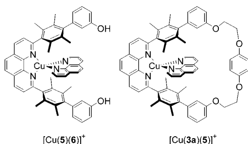
Figure 3. Two model complexes. For [\text{Cu}(\text{5})(\text{6})]^+ only the in-in isomer (with regard to the phenolic OH functionalities) is shown.
